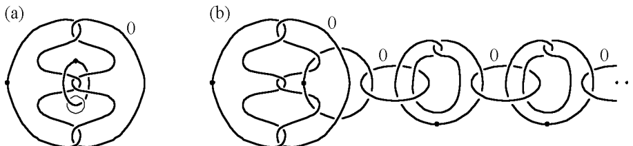
FIGURE 5. A small exotic R^4
