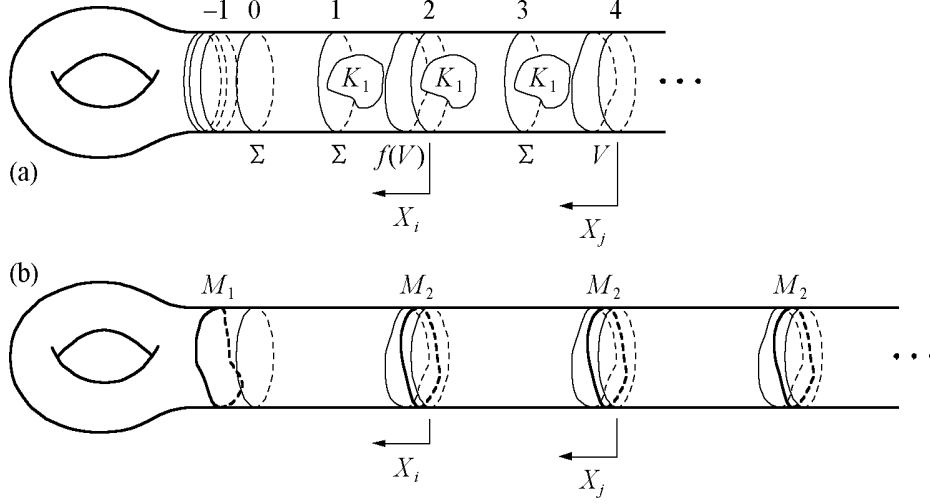
FIGURE 2. Corrupted end and periodic end
