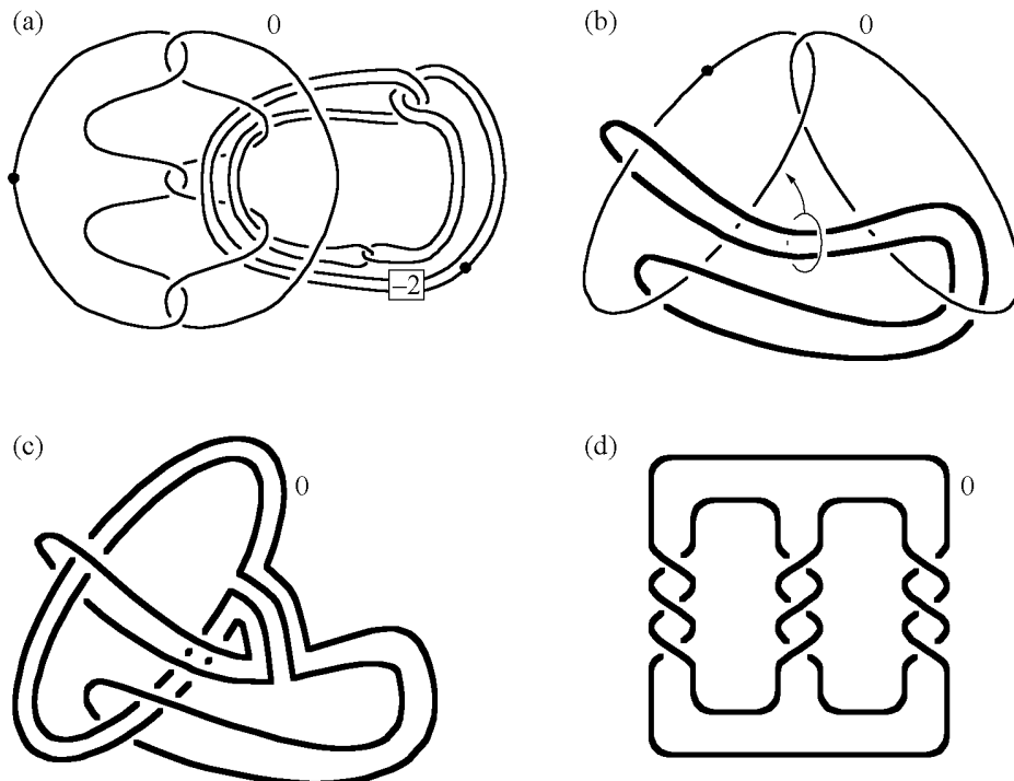
FIGURE 7. Calculation of the boundary of Y_n
