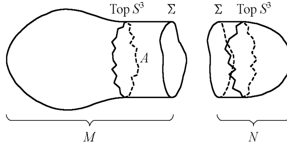
FIGURE 4. Any H_2 in A can be pushed into \Sigma .
