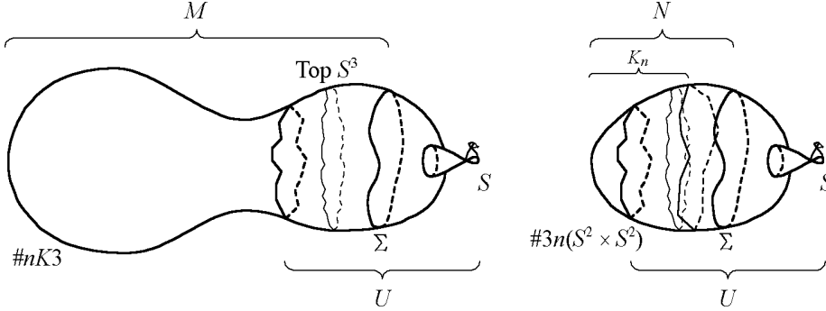
FIGURE 3. Calculation of e(R_n)
